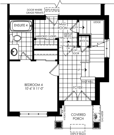
ELEVATION A OPT. 4 BEDROOM
